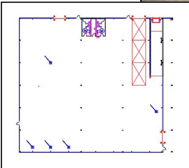
Advanced Blending Solutions floor plan
