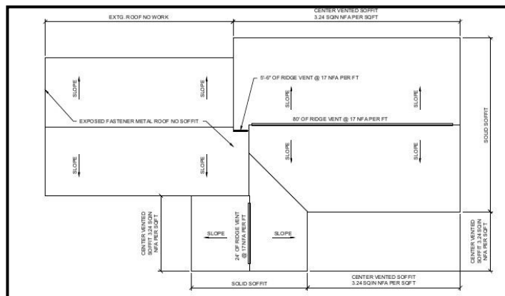
Roof plan.
