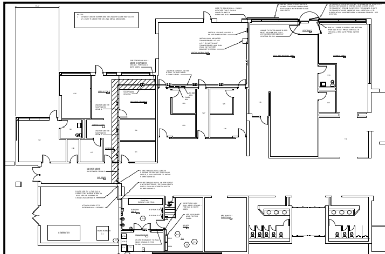
Floor plan for terminal and renovation plan.
