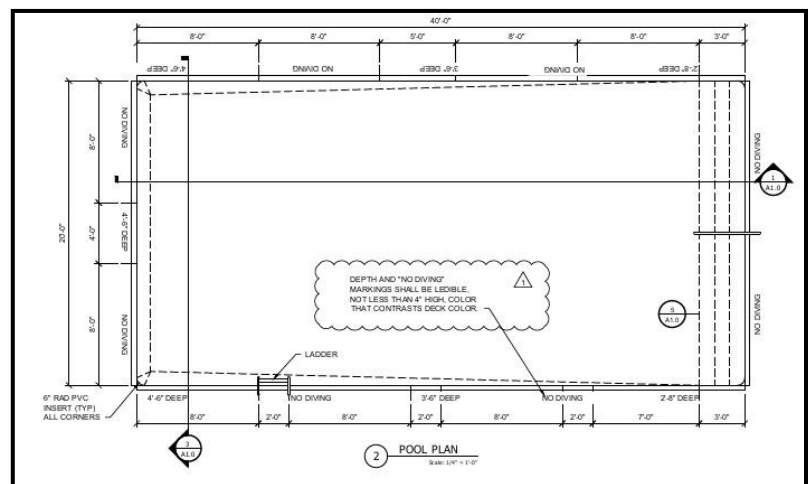
KOA swimming pool plan
