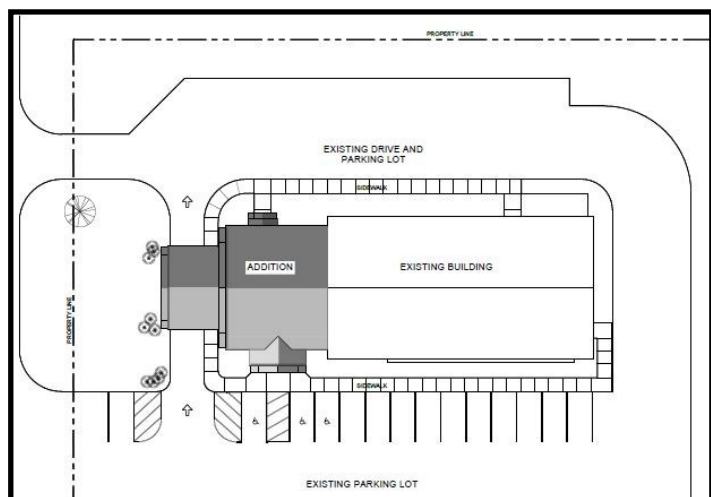
Proposed site plan with the new addition
