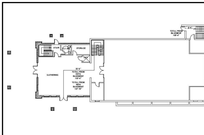
Proposed Main Level Floor Plan of the new addition
